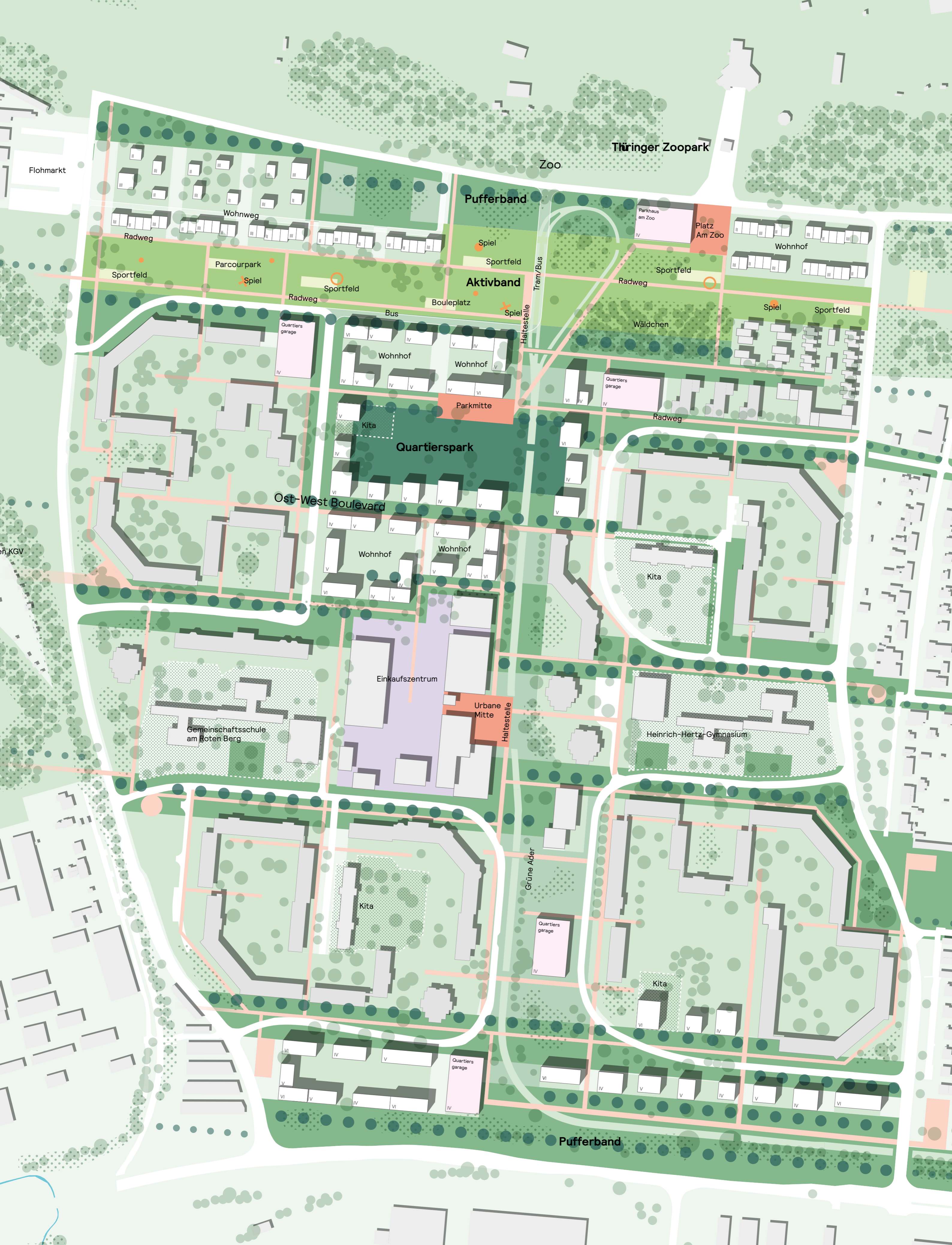
V3: 'Ost-West' // Lageplan M 1:2000
